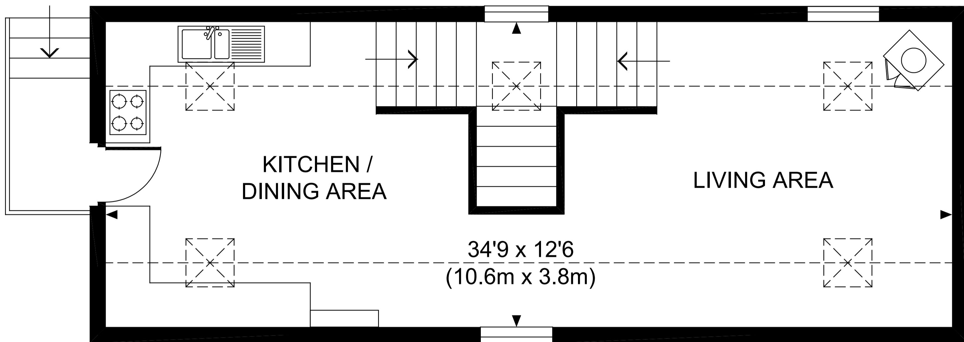
FIRST FLOOR
